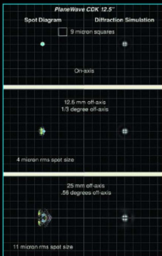
RGB = 720, 585, 430 nm Simulation is for a flat field.
